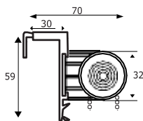
headrail (optional)
